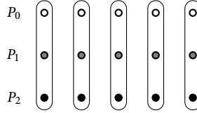
Figure 3.3. A horizontally coloured cliquy (3, 5) -grid
