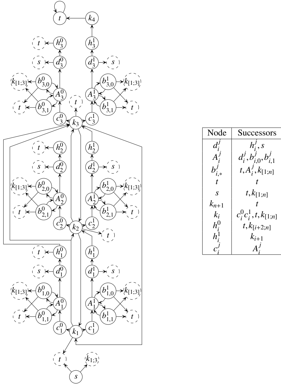
Figure 3: The graph \mathcal{Z}_3 and the edge relation of \mathcal{Z}_n for the counterexample to Zadeh's least-entered rule.
