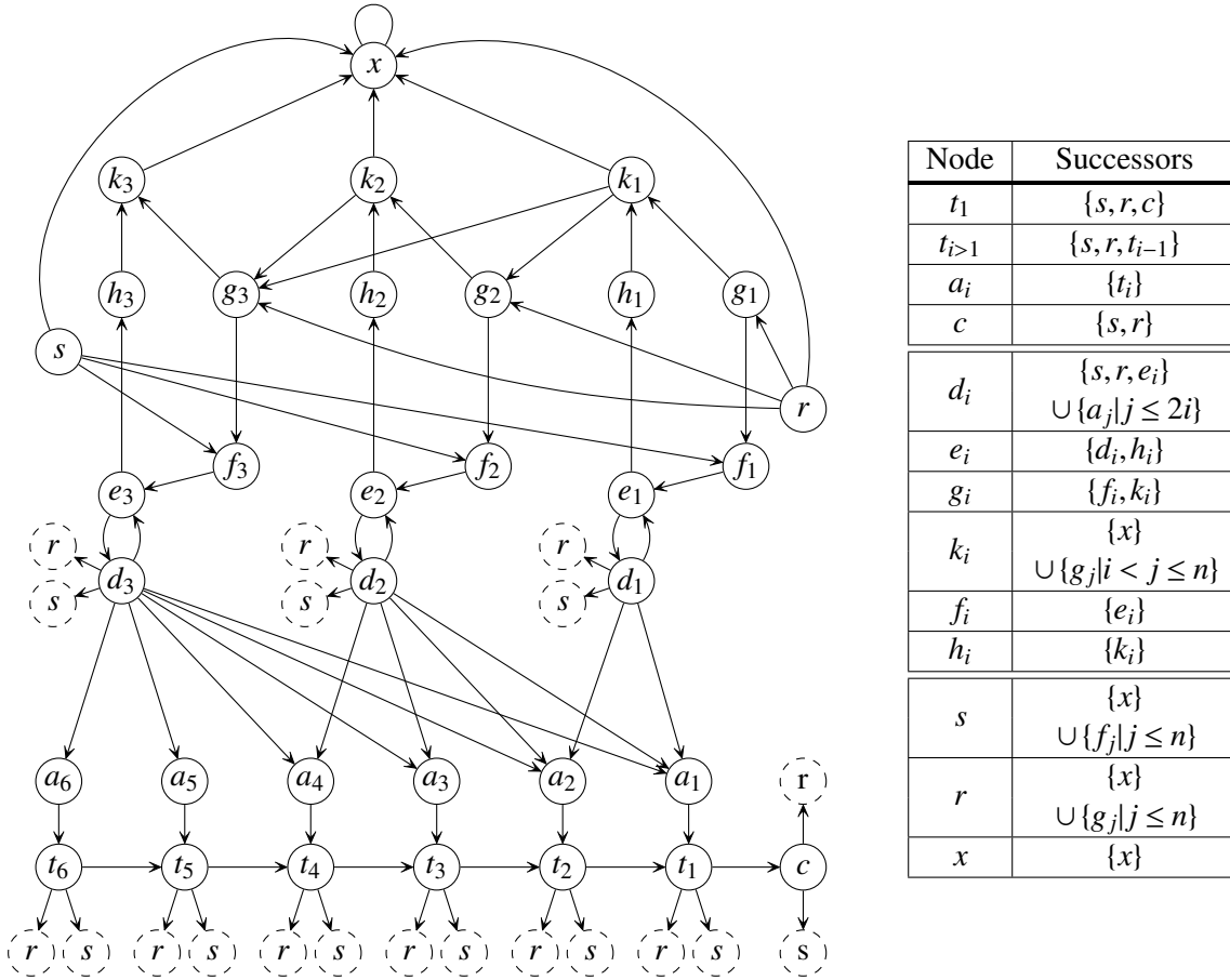
Figure 1: The graph \mathcal{G}_3 and the edge relation of \mathcal{G}_n for the counterexample to the switch-all rule.
